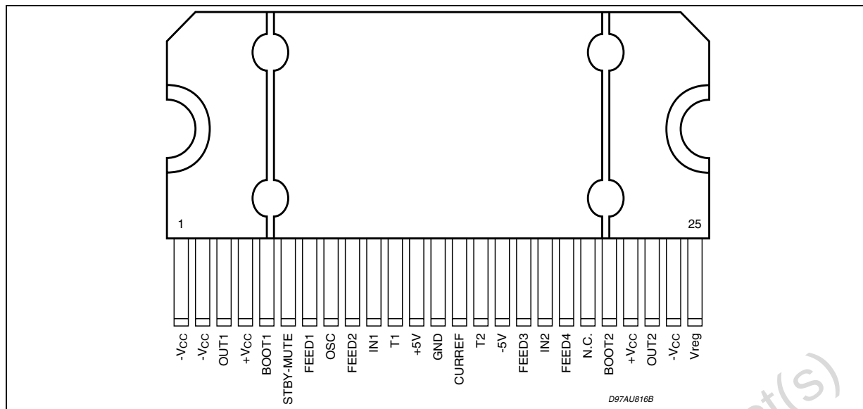
Figure 5. Pin Connection
