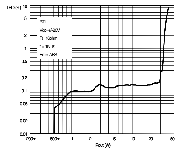
Figure 13. Distortion vs. Output Power in BTL
