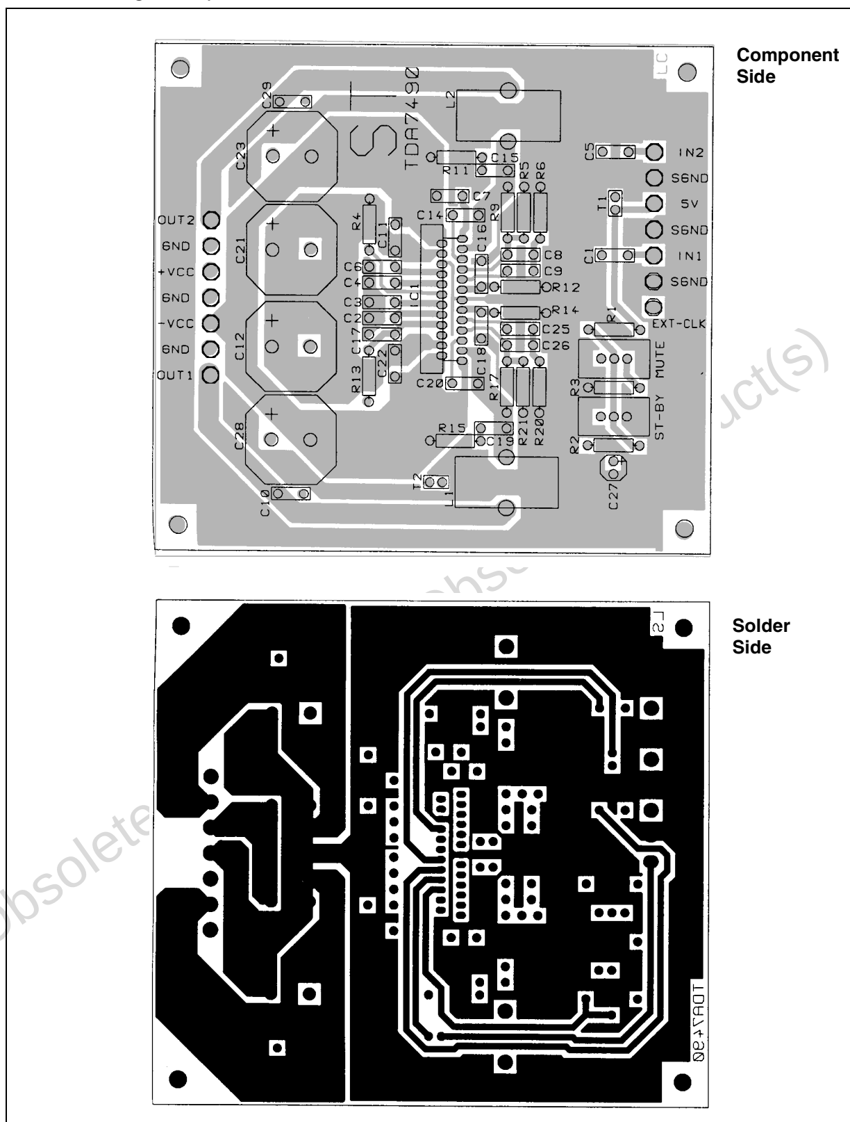
Figure 6. P.C. Board and Component Layout of the Figs. 2, 3 (for Stereo and Bridge Compatible Configuration)
