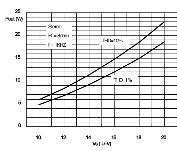
Figure 14. Pout vs Supply Voltage
